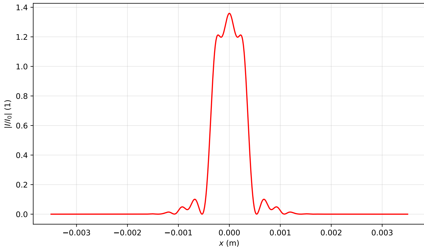
Intensity profile I(x, y = 0, z = 0.955)/I_0 , P_{in}=4.5P_{cr} , artificial time
